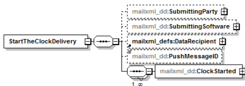
Figure 2.6: StartTheClockDelivery XSD Components
