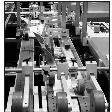
Plow Folding
