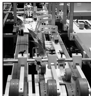
Plow Folding
