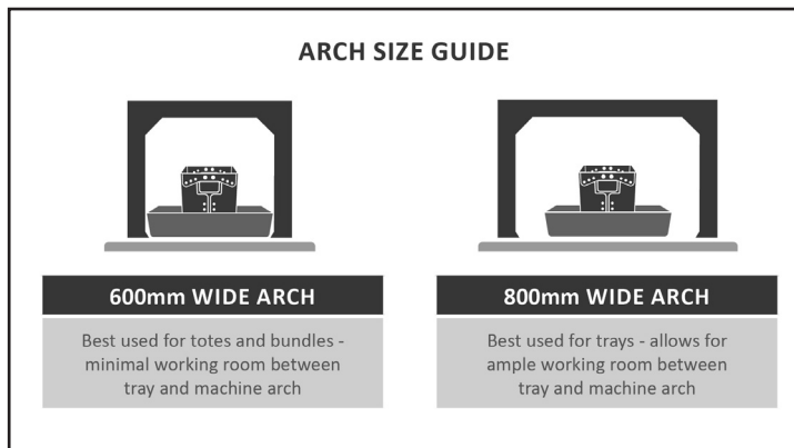
EAM-Mosca ROM-Fusion Walk Up, Operator Cycled Strapping Machine
